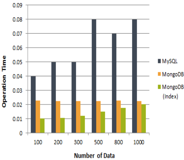
Fig. 1 Create Operation Execution Time Chart
