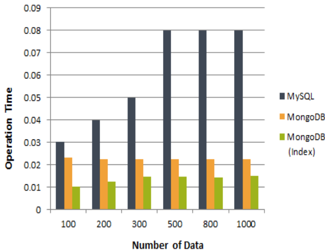
Fig.3 Update Operation Execution Time Chart
