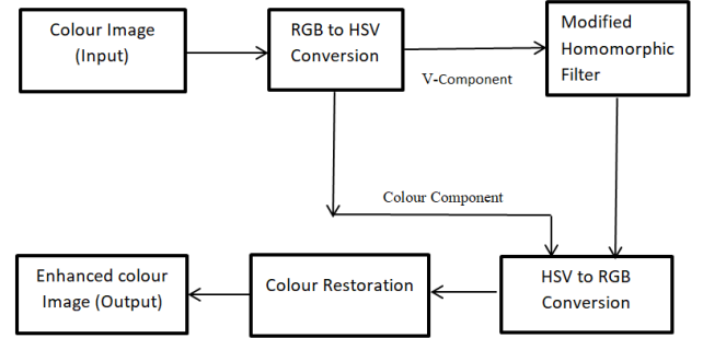
Fig. 4 Colour enhancement model for satellite imagery
