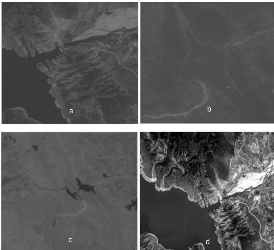
Fig. 5 Landsat8 Images for Chittoor region.(a) Noisy ( \sigma=5 ) (b) Noisy ( \sigma=10 ) (c) Noisy ( \sigma=20 ) (d) Denoised and enhanced image of the same scene
