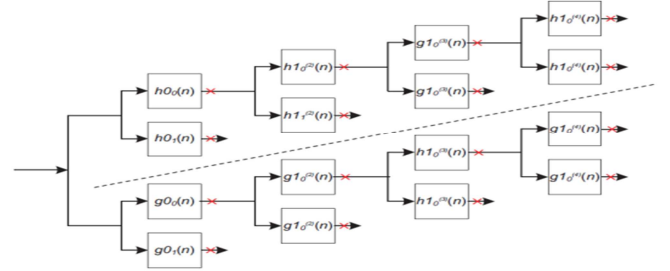
Fig. 1 Analysis stages of UDT-CWT. The crosses indicate the positions where down sampling would normally occur within the decimated DT-CWT
