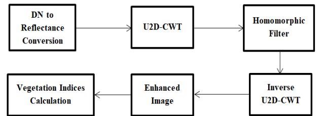
Fig. 2 Block diagram of proposed methodology
