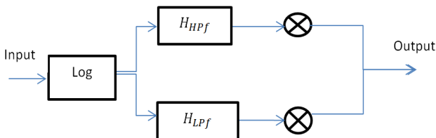
Fig. 3 Structure of modified homomorphic filter
