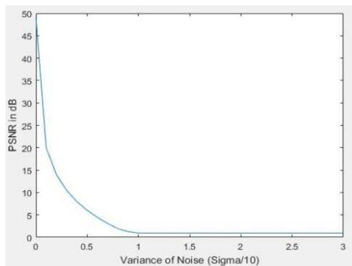
Fig. 6 Variations of PSNR with reference to Variance of the noise added
